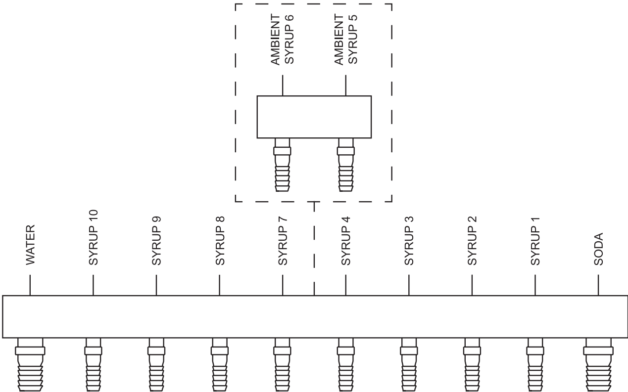
2300, 10 Valve, Standard Plumbing Diagram
