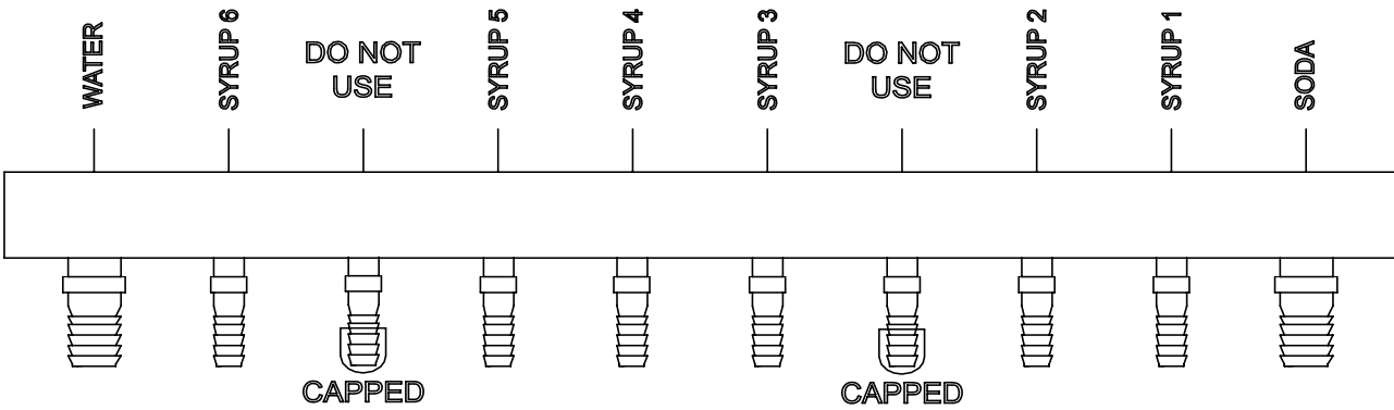
2300, 8 Valve, Standard Plumbing Diagram
