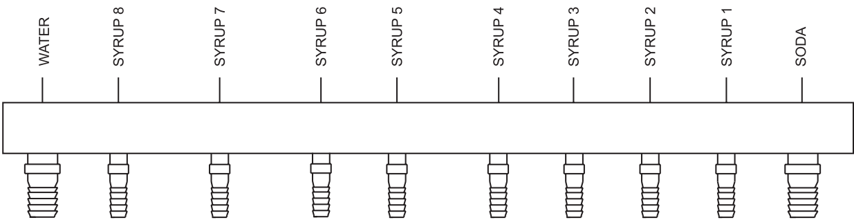
2300, 10 Valve, Standard Plumbing Diagram
