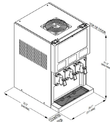
THREE FLAVOR 373 SERIES
