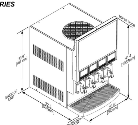
FOUR FLAVOR 774 SERIES
