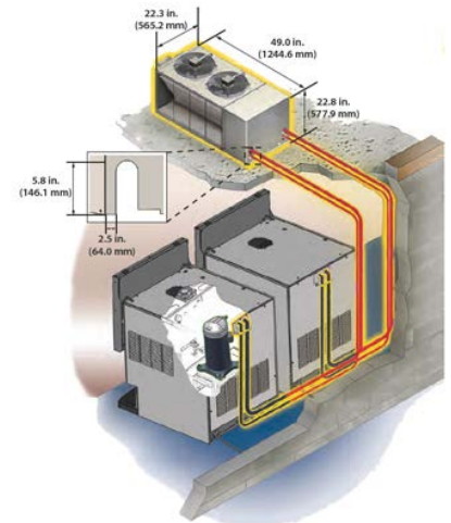
DUAL REMOTE CONDENSER
