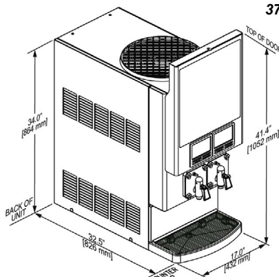
TWO FLAVOR 772 SERIES
