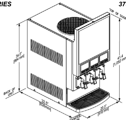
THREE FLAVOR 773 SERIES
